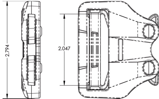
2" - 50mm Body Loop: 250-0021
