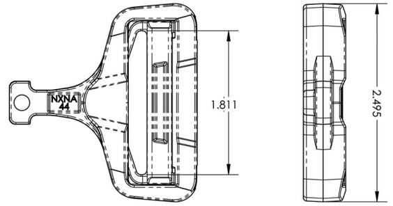
1 3/4" - 44mm Latch Loop: 250-0111
