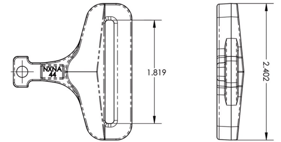
1 3/4" - 44mm Latch Loop: 250-0111
