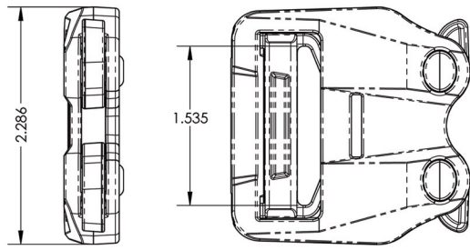
1 1/2" - 38mm Body Slider: 250-0002
