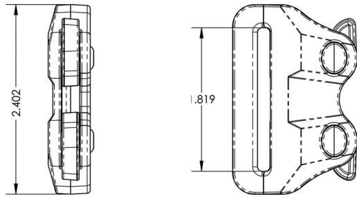
1 3/4" - 44mm Body Loop: 250-0011
