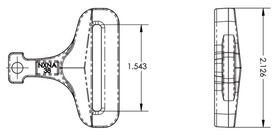
1 3/4" - 38mm Latch Loop: 250-0101
