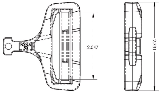
2" - 50mm Latch Loop: 250-0121
